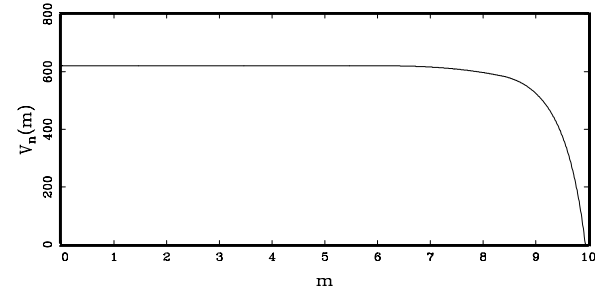
Figure 4.b V_n(m) \alpha = .6
