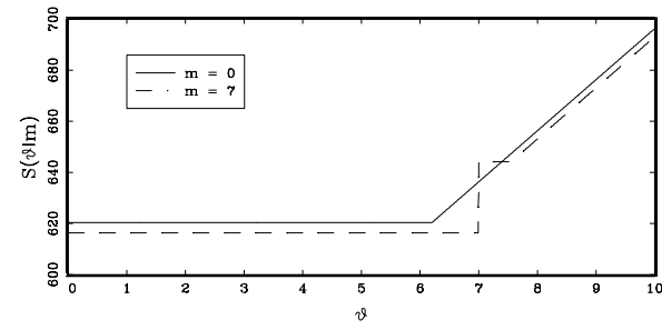
Figure 4.d S(\phi|m) \alpha = .6
