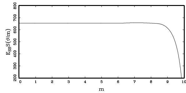
Figure 4.f E_{SS}S(\phi|m) \alpha = .6
