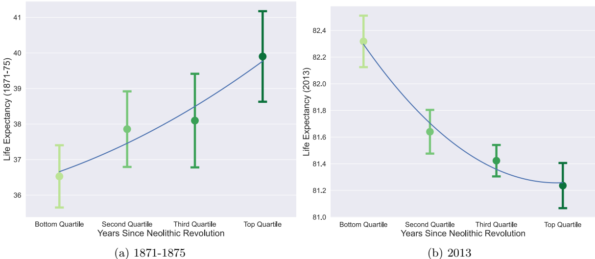
Figure 1: Life Expectancy Across French Départements before and after the Second Epidemiological Transition, conditional on the Timing of the Neolithic Revolution
