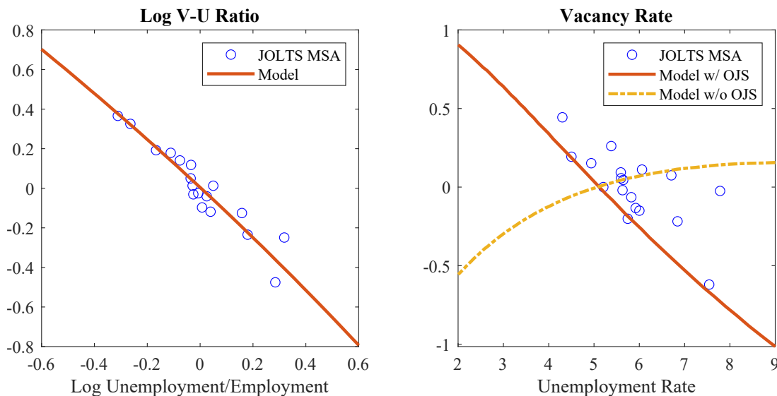
Figure 21: Model Predictions on Tightness and Spatial Beveridge Curve
