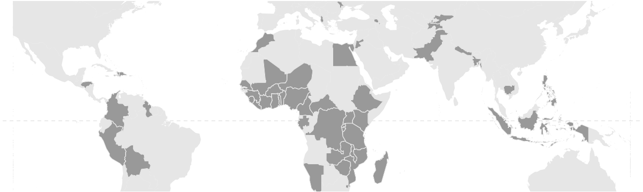
(B) Spatial incidence of hot days and high wet bulb (humidity-indexed temperature) days
