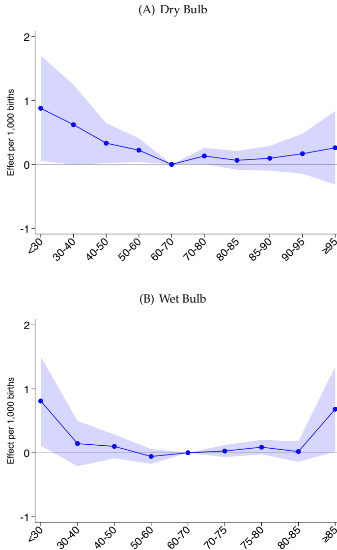
Figure 2: The Impacts of Wet and Dry Bulb Temperatures During Birth Month on Infant Mortality
