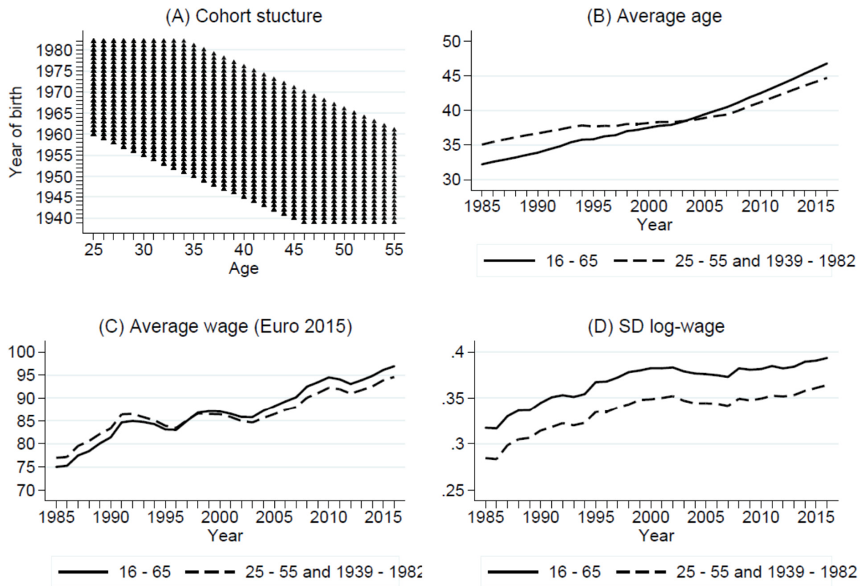
Figure 1: Descriptive statistics
