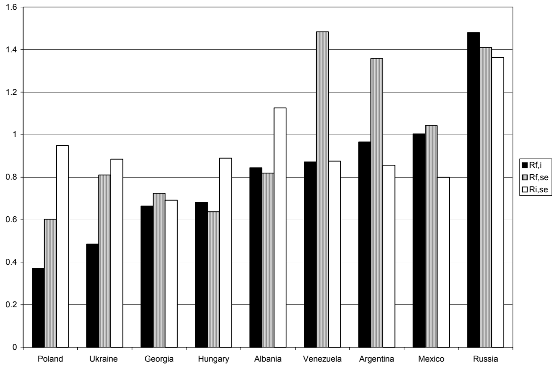
Figure 2: R indicators (The R indicator is the ratio T_{ij} / T_{ji} )
