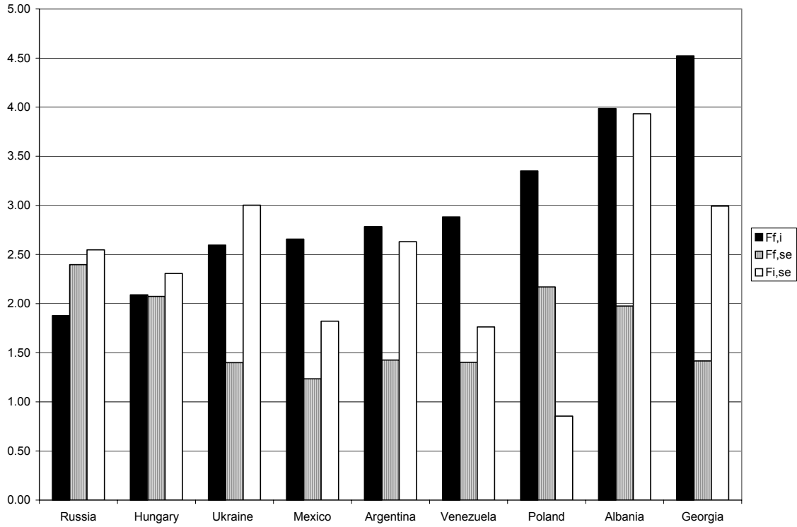
Figure 1: The F indicators of mobility (The F indicator is the sum of T_{ij} + T_{ji} )
